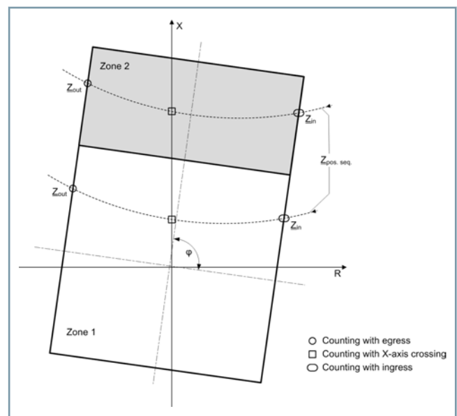
Figure 3.2/16 Impedance Zones for Out-of-Step Protection
