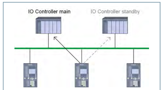
Figure 3.7/17 Connection of an Input/Output Device to 2 Different IO Controllers
