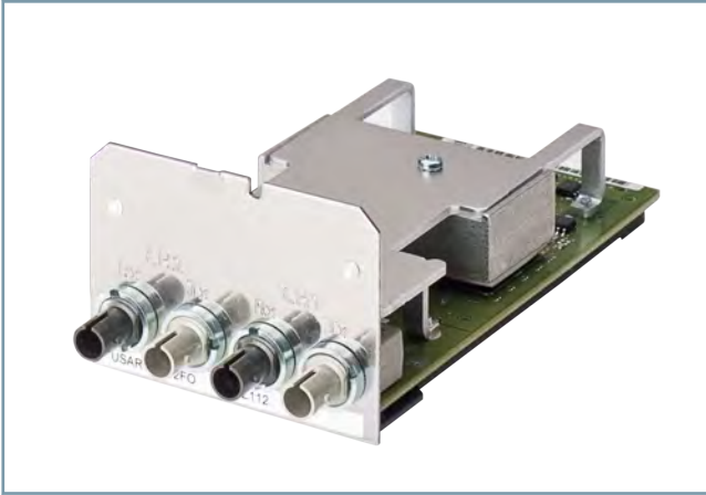
Figure 3.7/3 Serial Optical 820-nm Double Module (USART-AE-2FO)
