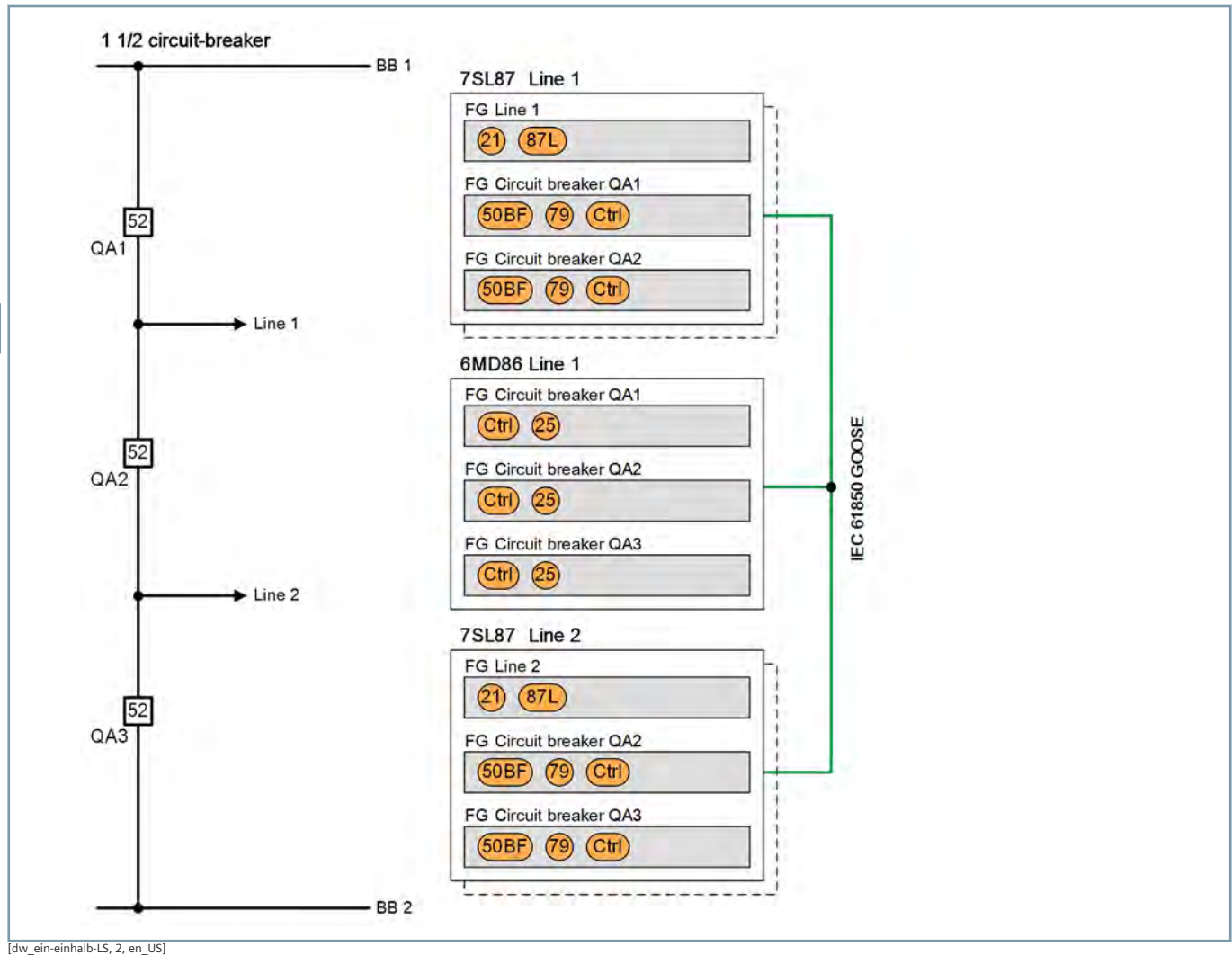
Figure 2.3/27 Modular and Decentralized Protection and Control Solution
