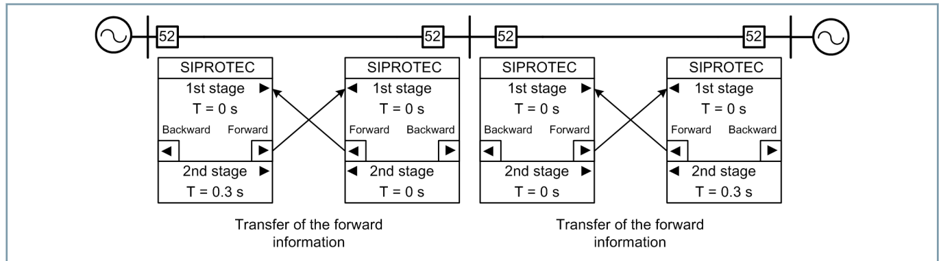
Figure 2.4/8 Application Example: Principle of Directional Comparison Protection for Power Line with an Infeed at Both Ends
