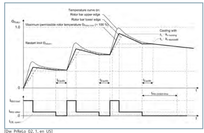
Figure 3.2/11 Temperature Curve of the Rotor and Repeated Attempts to Start the Motor
