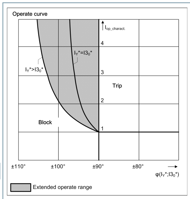
Figure 3.2/25 Operate Curve
