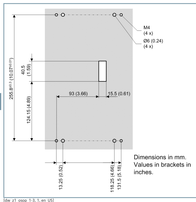
Figure 6.3/14 Drilling Pattern of the On-Site Operation Panel of the 1/3 Device
