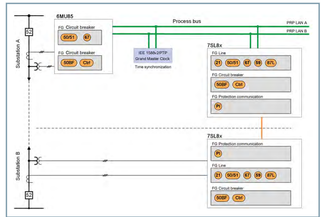
Figure 3.7/12 Line Differential Protection in Mixed Operation
