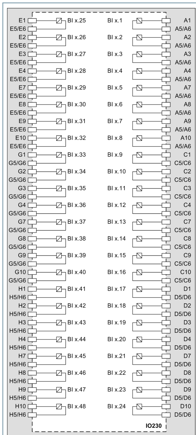
Figure 6.2/19 Connection Diagram IO230
