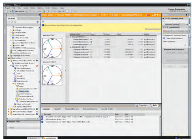
Figure 3.9/2 Display of Analog Measuring Points in Phasor Diagrams
