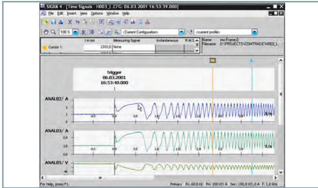
Figure 4.4/2 SIGRA Time Signals
