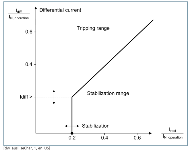
Figure 3.2/17 Operate Curves
