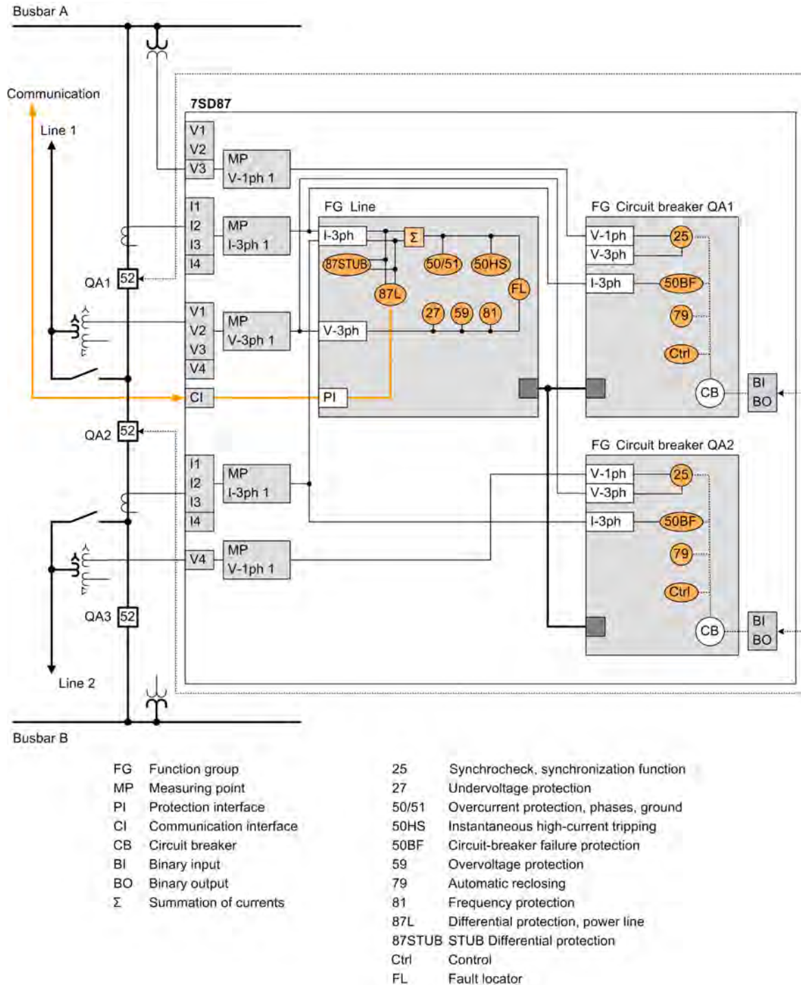
Figure 2.7/8 Application Example: Line Differential Protection for Overhead Line with Breaker-and-a-Half Layout
