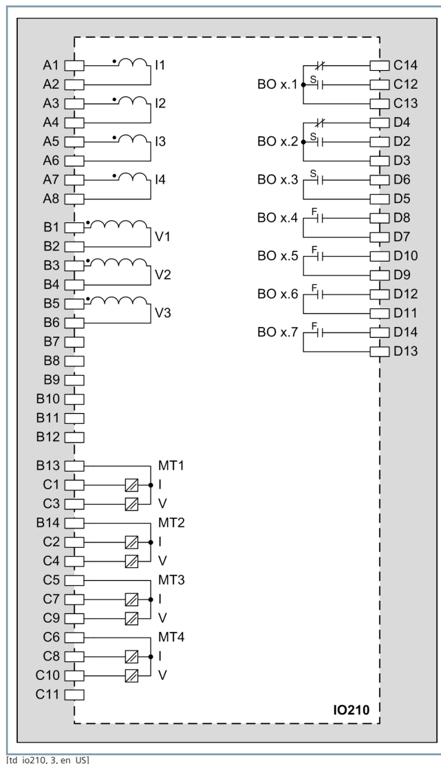
Figure 6.2/14 Connection Diagram IO210
