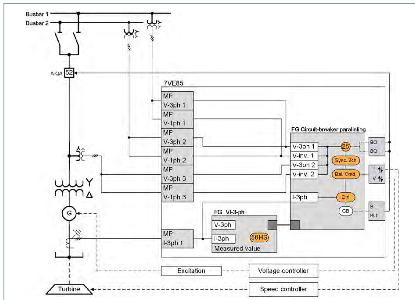
Figure 2.14/10 Application Template: Paralleling 2 Channels for 1 Synchronization Location with Voltage Selection and Balancing Commands 12 V, 4 I
