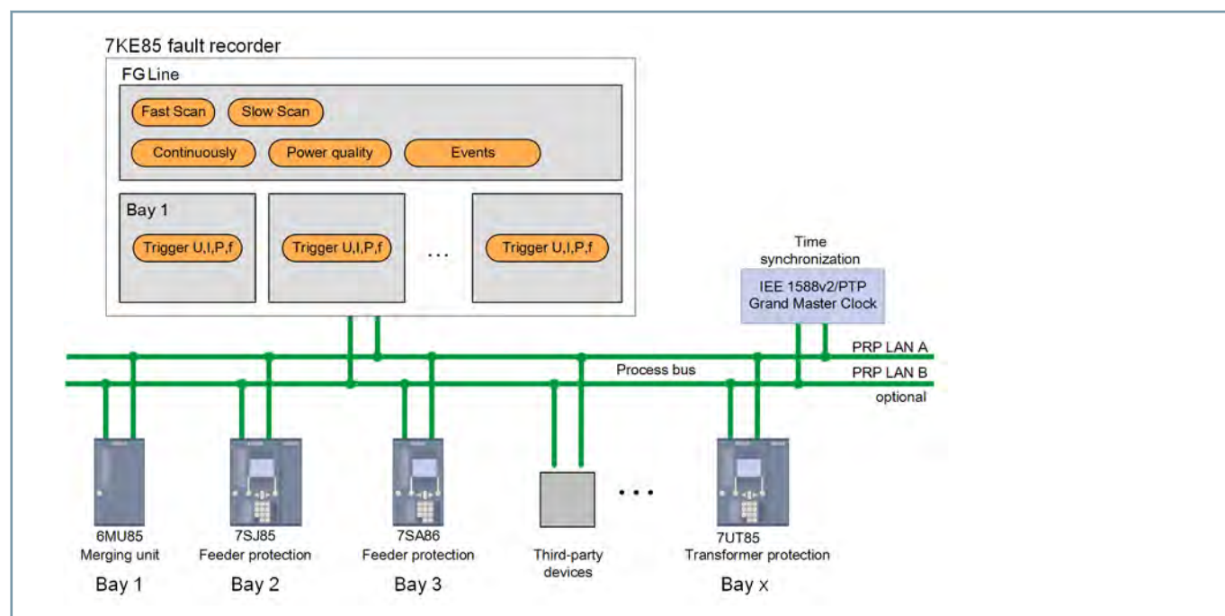
Figure 2.3/35 Decentralized Fault Recorder
