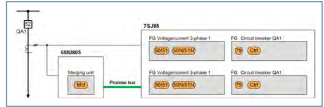
Figure 3.7/11 Parallel Operation of Conventional and Digital (Process Bus) Connection to an Instrument Transformer
