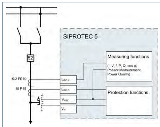
Figure 3.1/3 Connection of Bay Units to Instrument Transformers and Protection-Class Current Transformers
