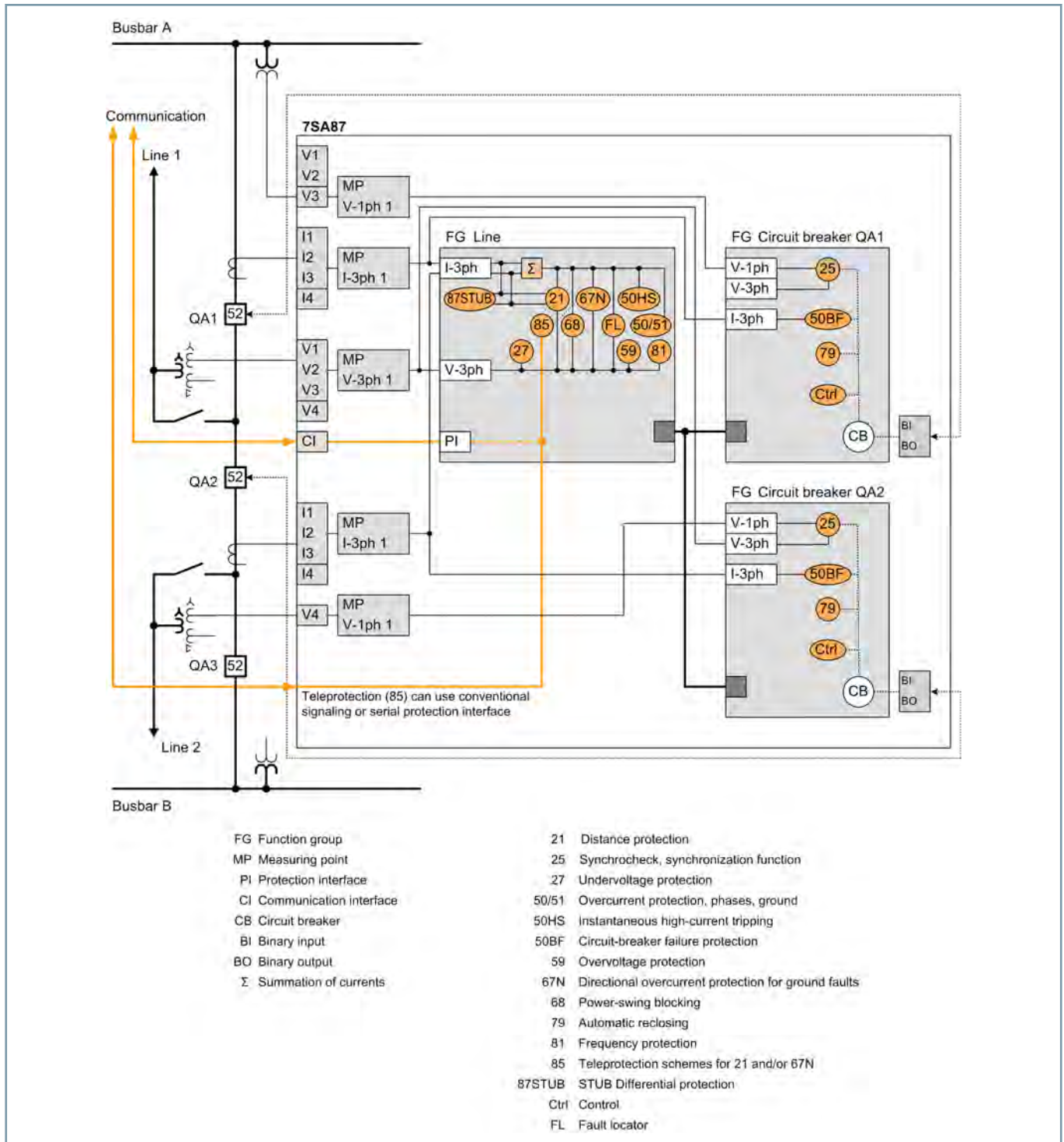
Figure 2.6/8 Application Example: Distance Protection for Overhead Line with Breaker-and-a-Half Layout
