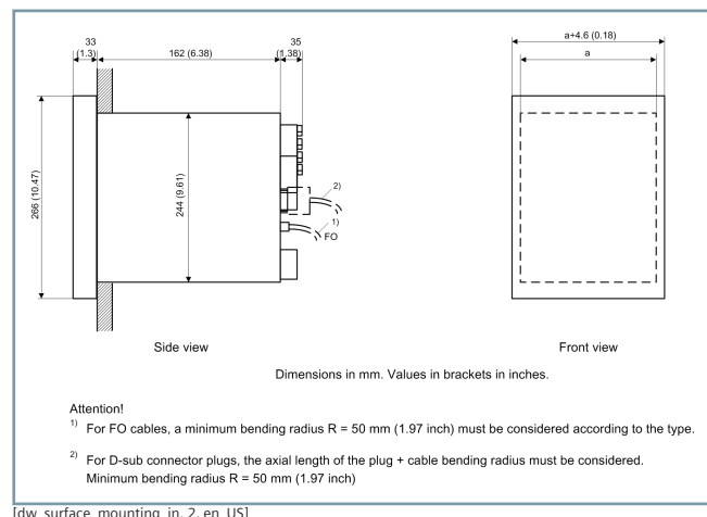
Figure 6.3/13 Flush-Mounting Devices, Dimensions from the Side and Front Views
