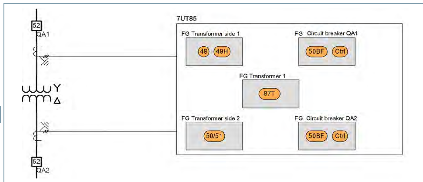
Figure 2.3/9 Two-Winding Transformer
