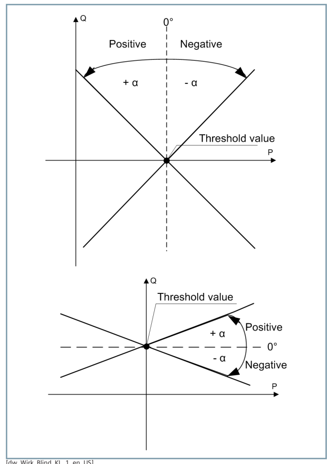
Figure 3.2/4 Active-Power Characteristic Curve and Reactive-Power Characteristic Curve
