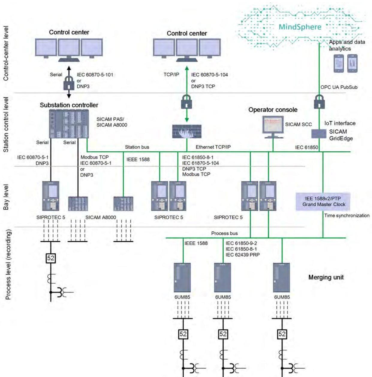
Figure 3.7/35 Communication Protocols in the Substation Automation Technology and in Network Control Systems
