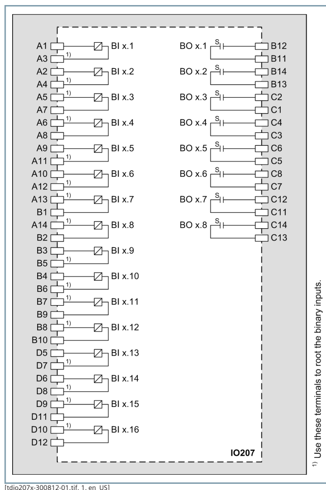
Figure 6.2/11 Connection Diagram IO207
