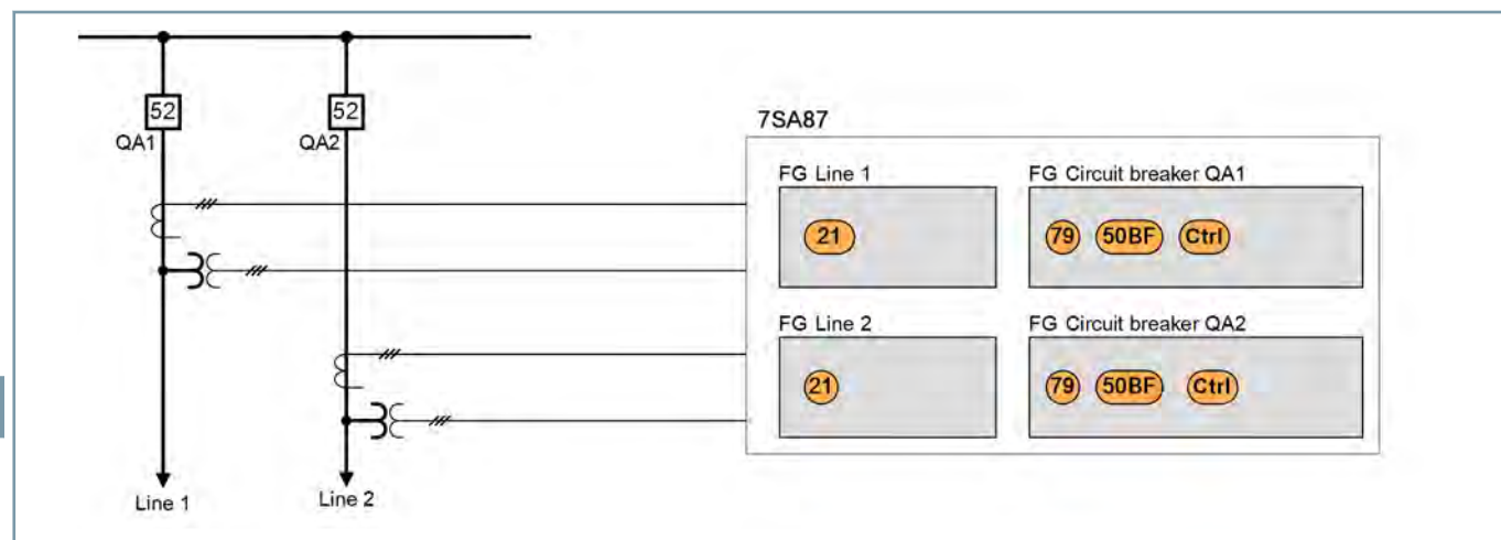
Figure 2.3/23 Distance Protection of 2 Parallel Lines with a Device
