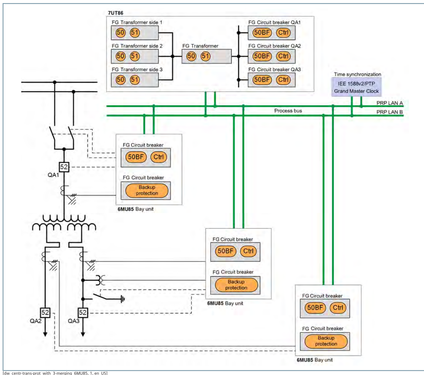
Figure 2.18/3 Centralized Transformer Protection with 3 6MU85 Merging Units
