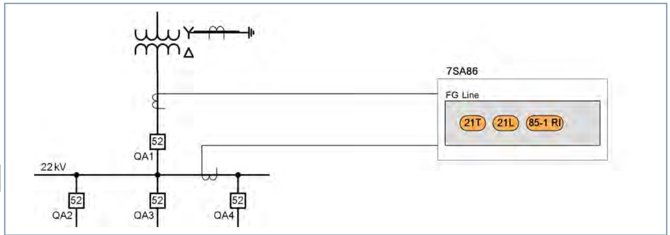
Figure 2.3/25 Impedance Protection
