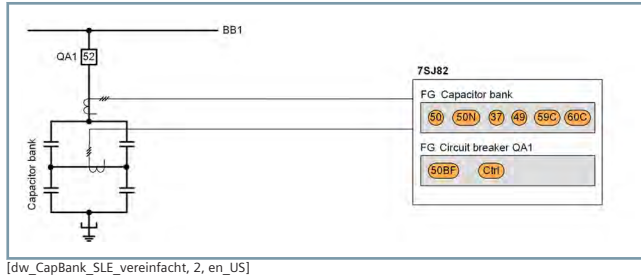
Figure 3.2/10 Protection of an H-Bridge Capacitor Bank
