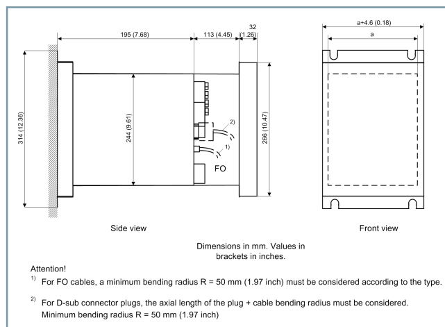
Figure 6.3/22 1/3 Surface-Mounted Device with Integrated On-Site Operation Panel, Dimensions in the Side and Front Views
