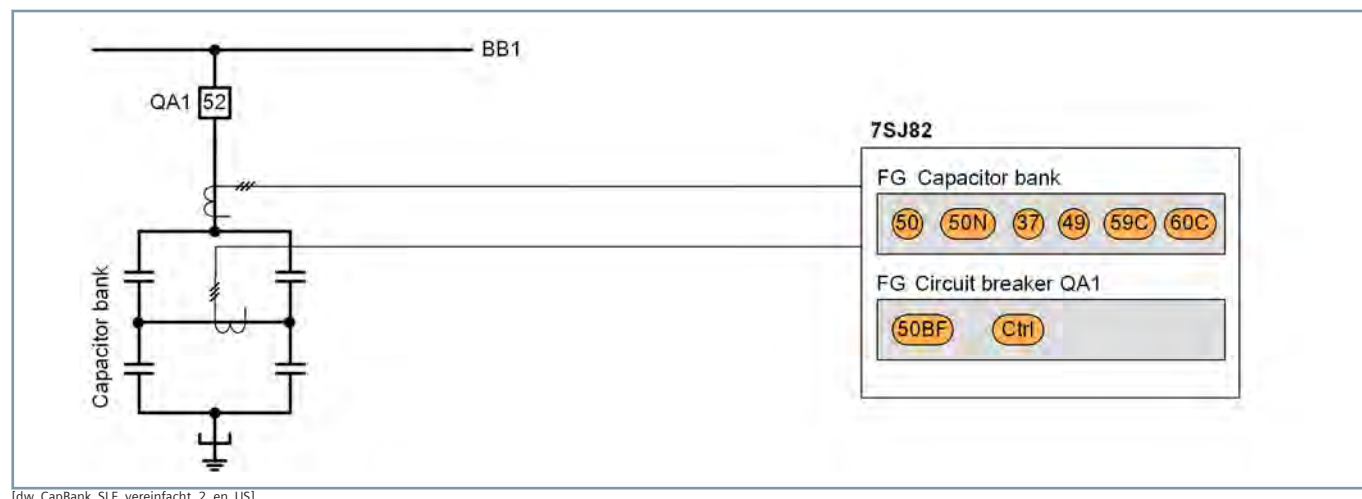
Figure 2.3/30 Protection of a Capacitor Bank in H-Bridge Connection
