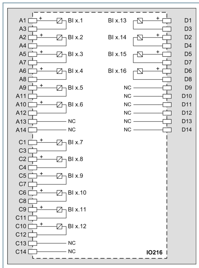
Figure 6.2/18 Connection Diagram IO216
