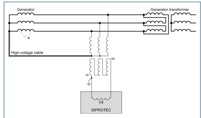
Figure 3.2/9 Implementation Example
