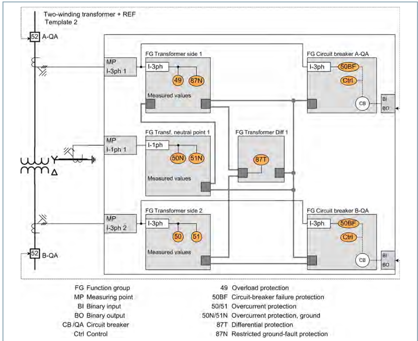
Figure 3.1/2 Transformer Protection
