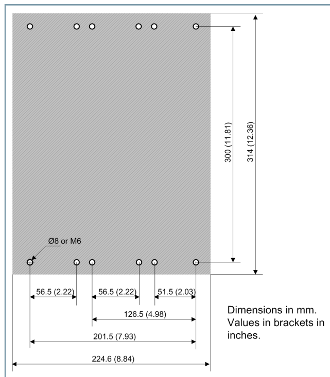
Figure 6.3/29 Drilling Pattern of a 1/2 Surface-Mounted Device – 2nd Device Row
