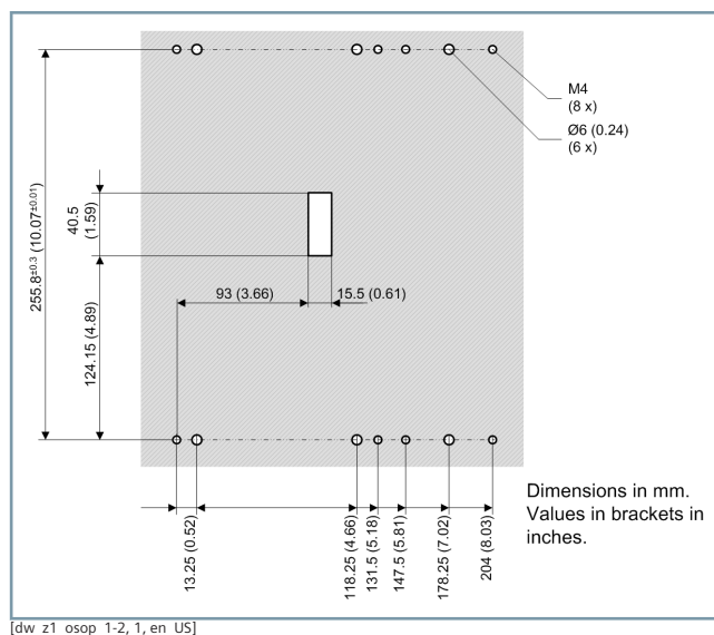
Figure 6.3/15 Drilling Pattern of the On-Site Operation Panel of the 1/2 Device
