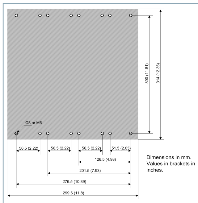
Figure 6.3/30 Drilling Pattern of a 2/3 Surface-Mounted Device – 2nd Device Row
