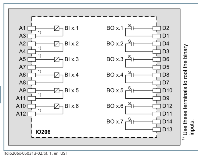
Figure 6.2/10 Connection Diagram IO206
