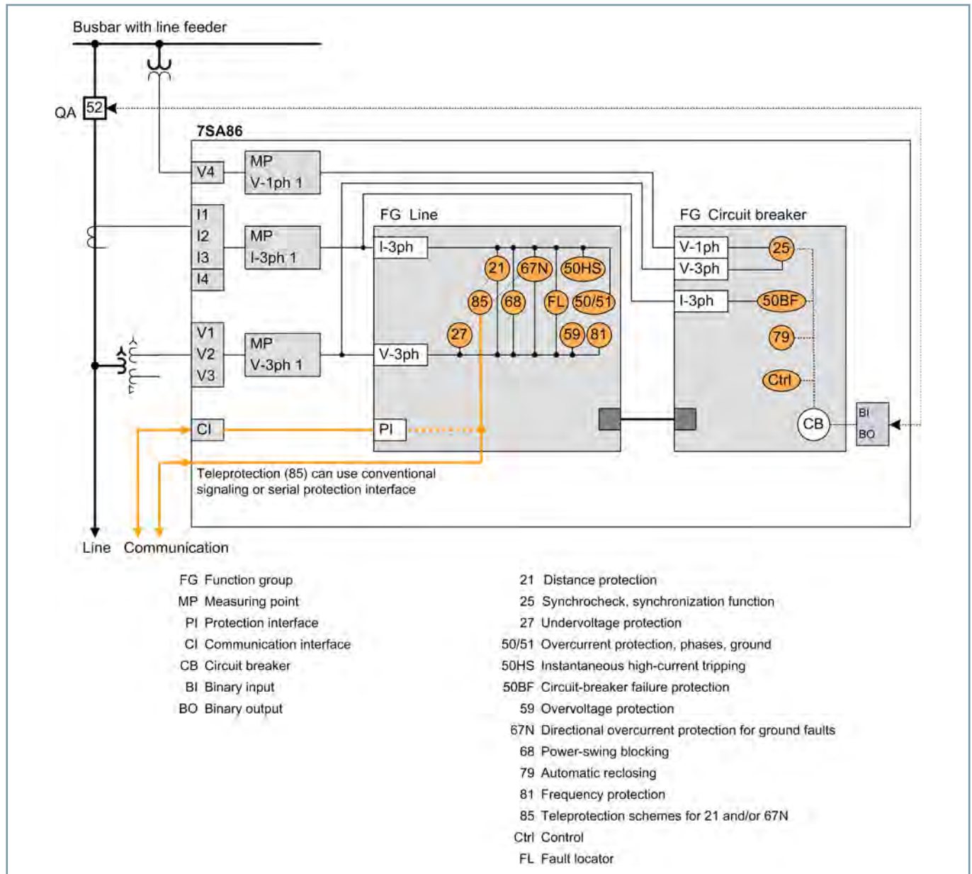
Figure 2.6/4 Application Example: Distance Protection for Overhead Line
