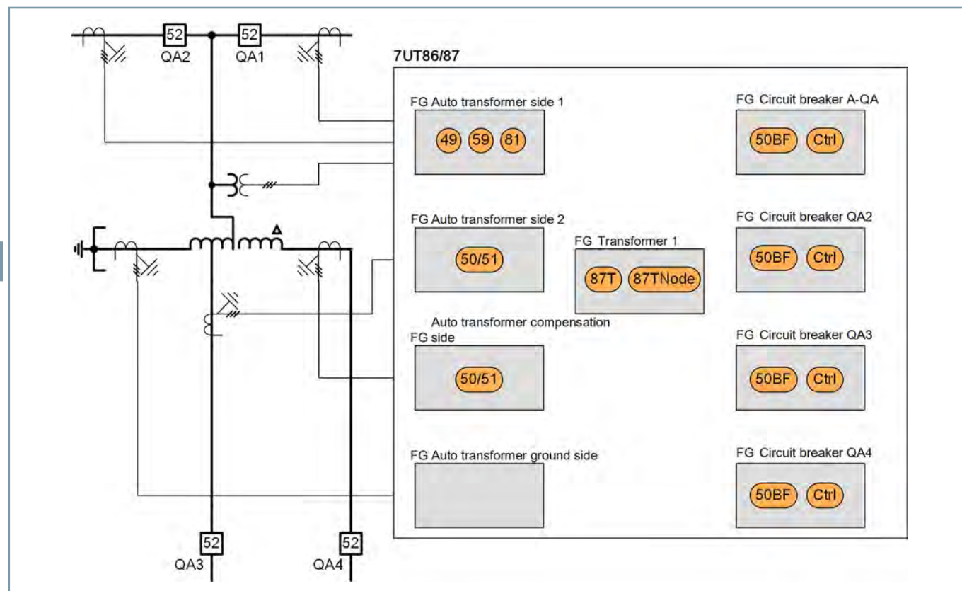
Figure 2.3/11 Auto-Transformer Bank
