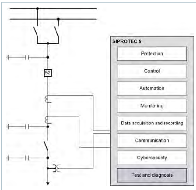
Figure 3.9/1 SIPROTEC 5 – Functional Integration – Test
