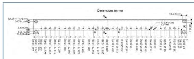
Figure 6.3/20 Angle Rail with Assembly Dimensions
