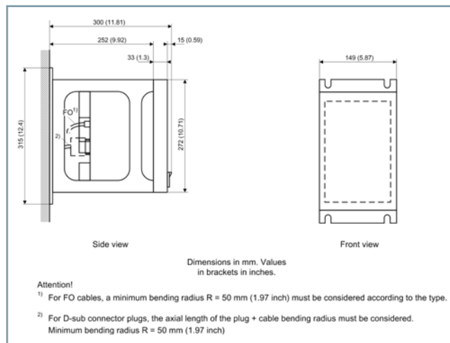
Figure 6.3/21 Non-Modular Surface-Mounted Device with Integrated On-Site Operation Panel, Dimensions from the Side and Front Views
