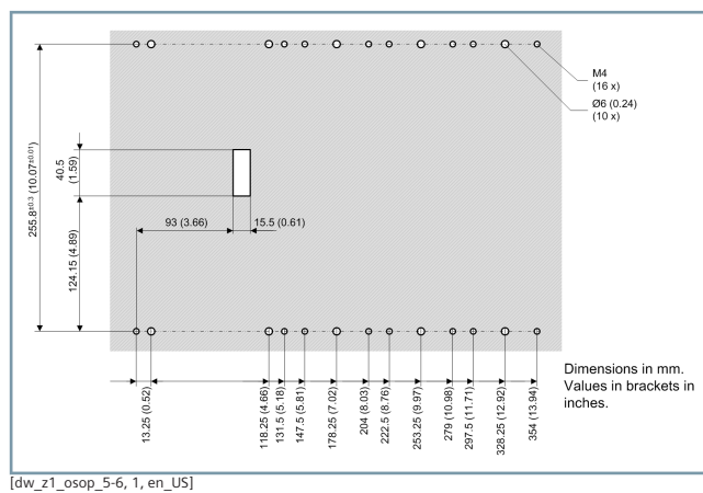
Figure 6.3/17 Drilling Pattern of the On-Site Operation Panel of the 5/6 Device
