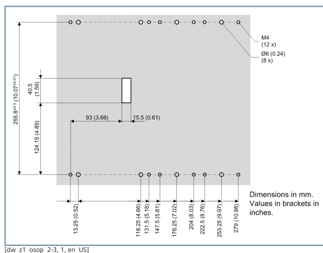
Figure 6.3/16 Drilling Pattern of the On-Site Operation Panel of the 2/3 Device
